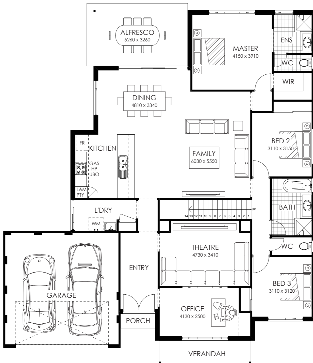
FLOOR PLAN
